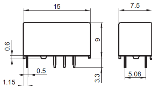
Outline Dimensions
